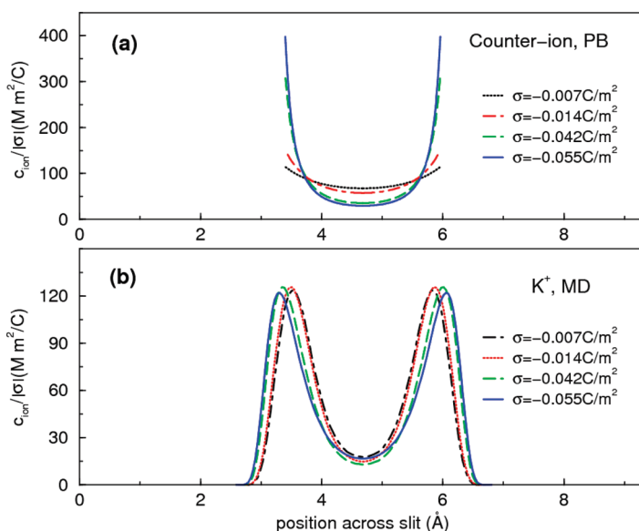
Figure 3. Variation of counterion (K + ion) concentration scaled by the slit wall charge density ( c_{\text{ion}}/|\sigma| ) in 9.36 Å-wide slits with different surface charge densities. (a) Prediction by the PB equation. The closest approach of the K + ion to the slit wall was taken as 3.3 Å. The solution dielectric constant was taken as 3.33, the same as the result of fitting the sandwich capacitor model (in Figures 4 and 5) to the capacitance data obtained from micropores immersed in 6 M KOH electrolytes. 6 (b) Prediction by the MD simulations.
