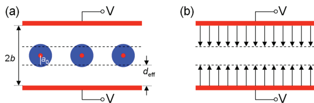
Figure 5. (a) Schematic of a sandwich capacitor formed by a layer of counterions located exactly midway between two electrodes with the same polarity and separated by W = 2b . (b) The equivalent system shown with the electric field lines. The locations of the dashed lines indicate the effective ion radius a_0 of the counterions, which is dictated by the spread of electron cloud (ref 11). The effective separation between the electrode surface and the counterions is d_{\text{eff}} .
