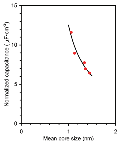
Figure 6. Experimental data (solid dots) in ref 6 of microporous activated carbon electrode materials in a 6 M aqueous KOH electrolyte fit with the sandwich capacitance model (solid curve) shown in eq 3.
