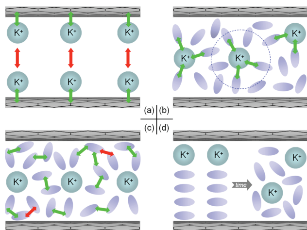
Figure 2. Schematic diagrams of the five factors, as described in the text, governing the distributions of the K^+ counterions in electrified slit-shaped micropores: (a) the long-range electrostatic ion–ion repulsion which drives ions toward the slit walls (factor 1) and the non-electrostatic ion-slit wall attraction (factor 2), indicated by the red and green double-headed arrows, respectively (color codes also applicable in the following); (b) the hydration of ions (factor 3), which drives ions toward positions to maximize their interactions with the hydration water molecules (the blue dashed circle indicates the primary hydration shell of one ion; compared to the ions in the slit center, the ion near the slit wall has smaller number of hydration water molecules); (c) the interaction between an ion's hydration water molecules with their surrounding water molecules (factor 4); and (d) entropic effects that drive the ordered distribution shown on the left toward a uniform/disordered distribution on the right (factor 5).
