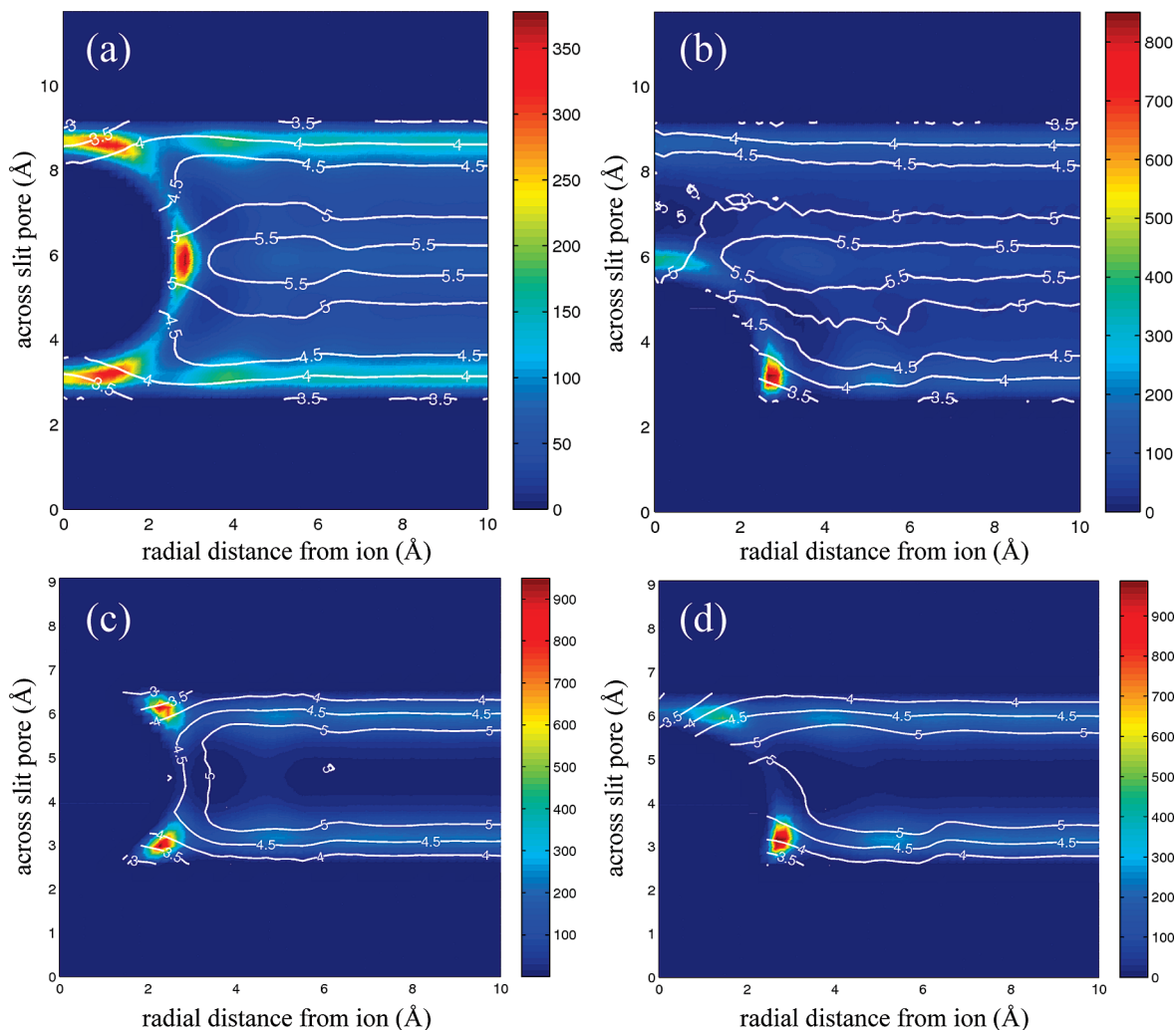
Figure 4. Distribution of water molecules around a K + ion located at different positions in slit pores (shown as different colors) and the coordination number of these water molecules (shown as contour lines): (a) K + located at z = 6.03 \text{ \AA} inside a 12.03 \text{ \AA} -wide slit pore; (b) K + located at z = 3.30 \text{ \AA} inside a 12.03 \text{ \AA} -wide slit pore; (c) K + located at z = 4.68 \text{ \AA} inside a 9.36 \text{ \AA} -wide slit pore; (d) K + located at z = 3.30 \text{ \AA} inside a 9.36 \text{ \AA} -wide slit pore.
