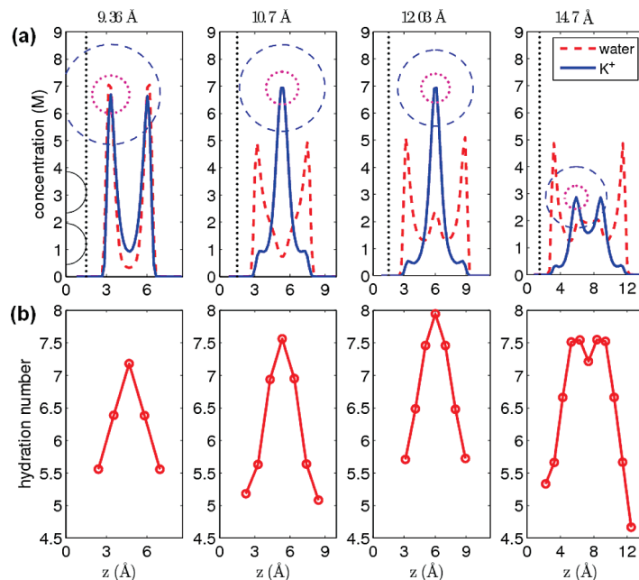
Figure 1. (a) Concentration profiles of water and K + ions inside slit pores with various widths. For clarity, the water concentration has been divided by a factor of 30. The concentric circles denote the size of bare and hydrated K + ions. The hemicircles in the leftmost figure denote the van der Waals radius of the wall atom, and the dashed line denotes the effective boundary of the lower wall. (b) Hydration number of K + ions across slit pores with various widths. All slit walls have the same surface charge density of \sigma = -0.055 \text{ C/m}^2 .
